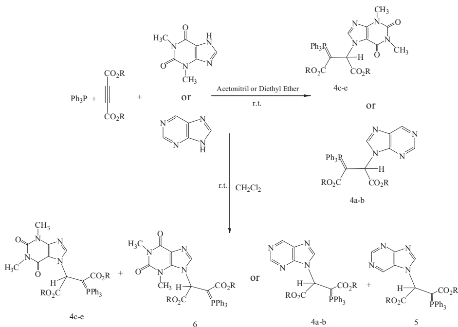
Figure 3 Synthesis of stable phosphorus ylide from purine and theophylline in different solvents.
