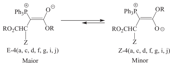
Figure 2 Equilibrium could appear between E and Z isomer.
