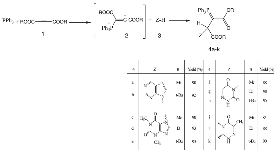
Figure 1 Synthesis of stable phosphorus ylides 4a–k .
